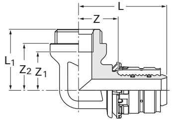
MLC-S Male/Female Press 90° Elbow
