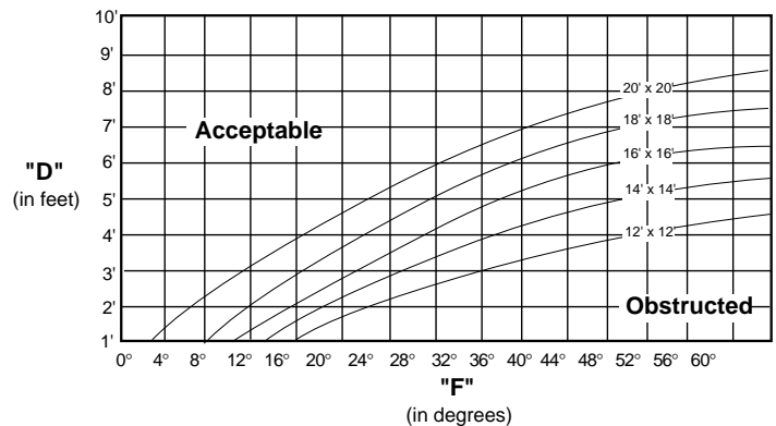
Figure 8 Graph
