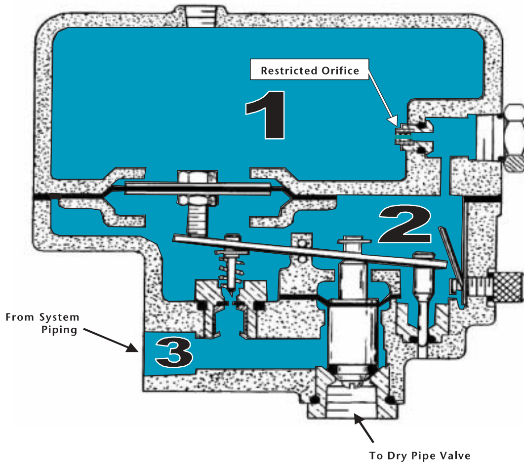
Figure 3 - Section View of a Mechanical Accelerator
