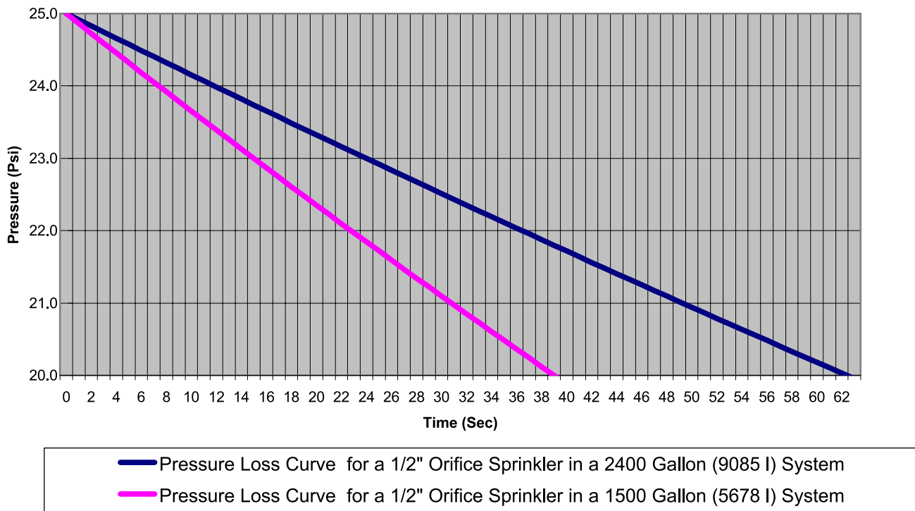
Figure 1- Air Loss Curves
