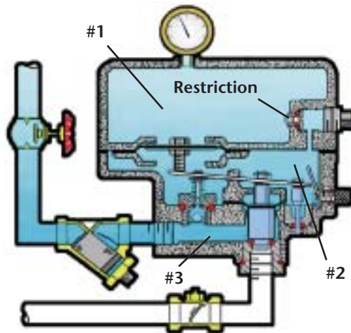
Figure 4 - Section View of a Mechanical Accelerator in the Set Position
