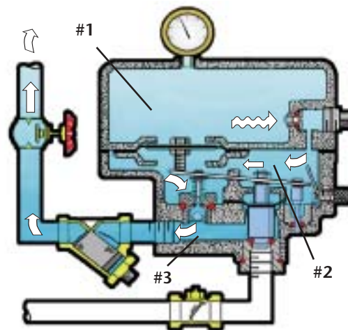
Figure 5 - Air Movement In a Mechanical Accelerator Upon Sprinkler Activation
