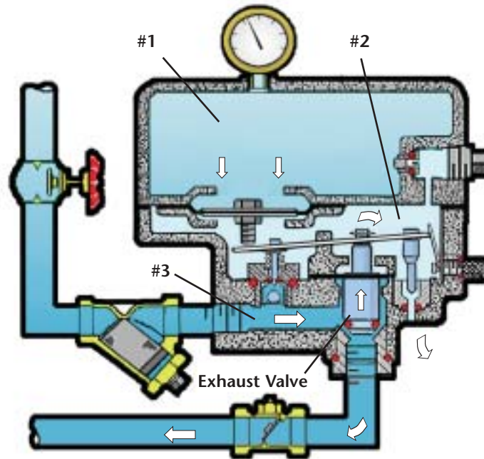
Figure 6 - Upon 2 psi Differential Pressure (Chamber 1 & 2) - Accelerator Trips
