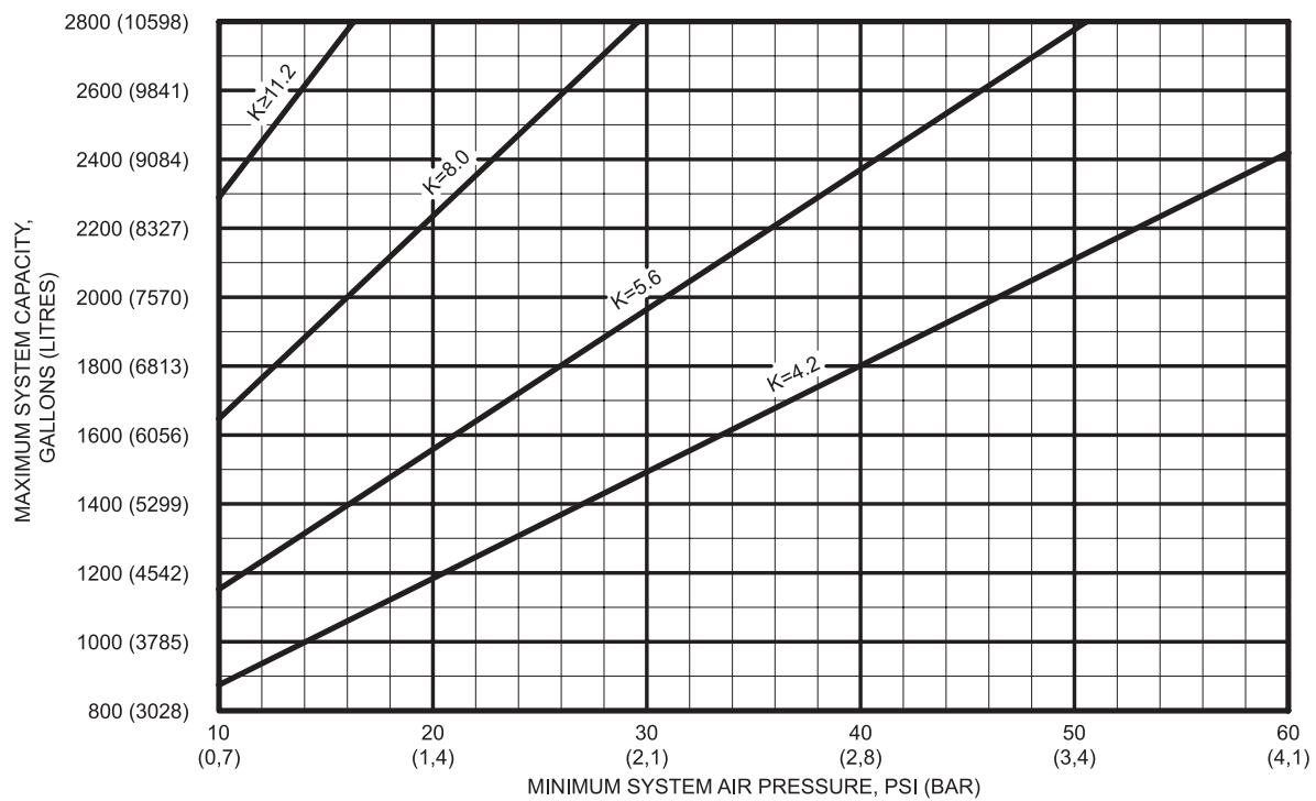
Figure 12 - K Factors That Result in 0.1 psi (0.007 bar) Drop/Second
