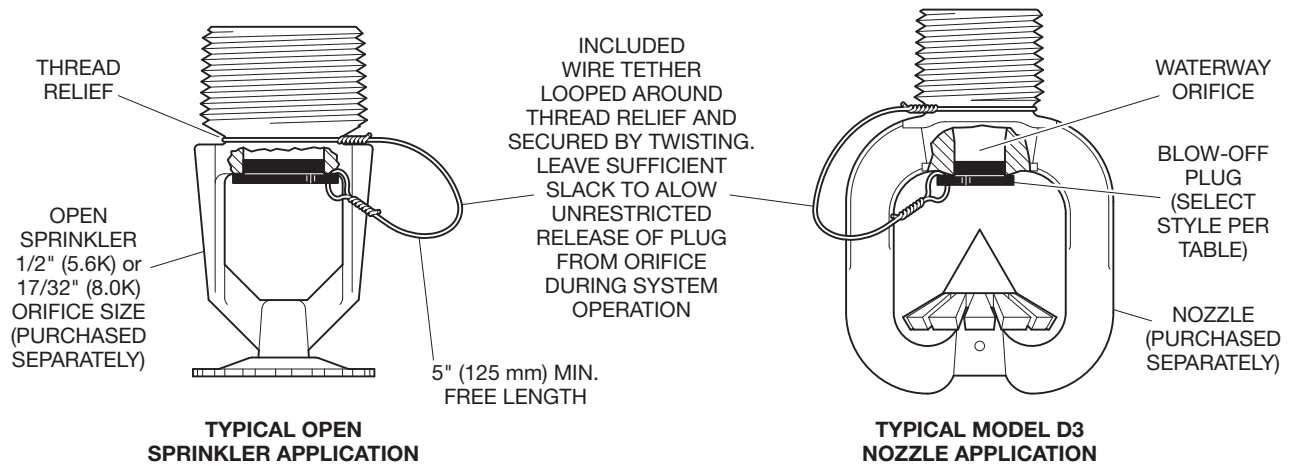
FIGURE 1 BLOW-OFF PLUGS
